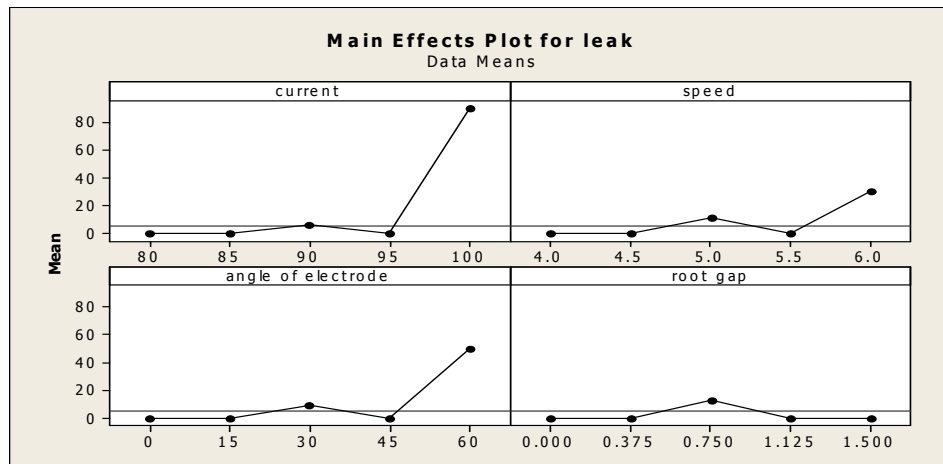
Fig. 5 Variations of average leak rate with mean values of factors
