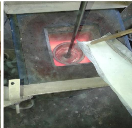
Fig. 1 b. Preparation of sample by stir casting
